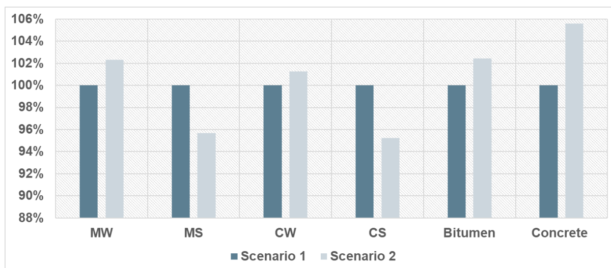
Figure 17: PED for the 2 scenarios for each roof system
