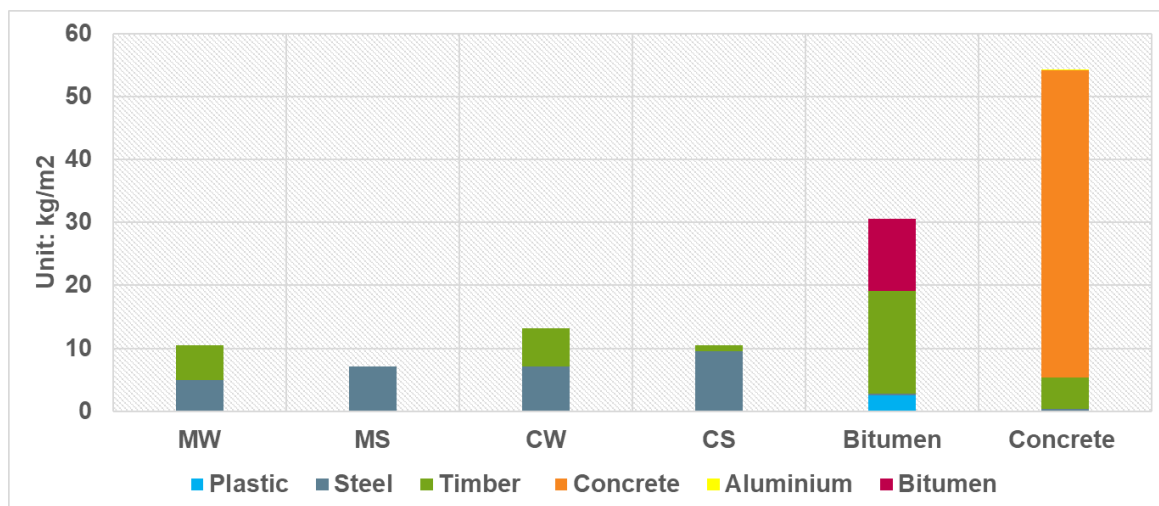
Figure 6: Mass composition per m² of the roof designs
