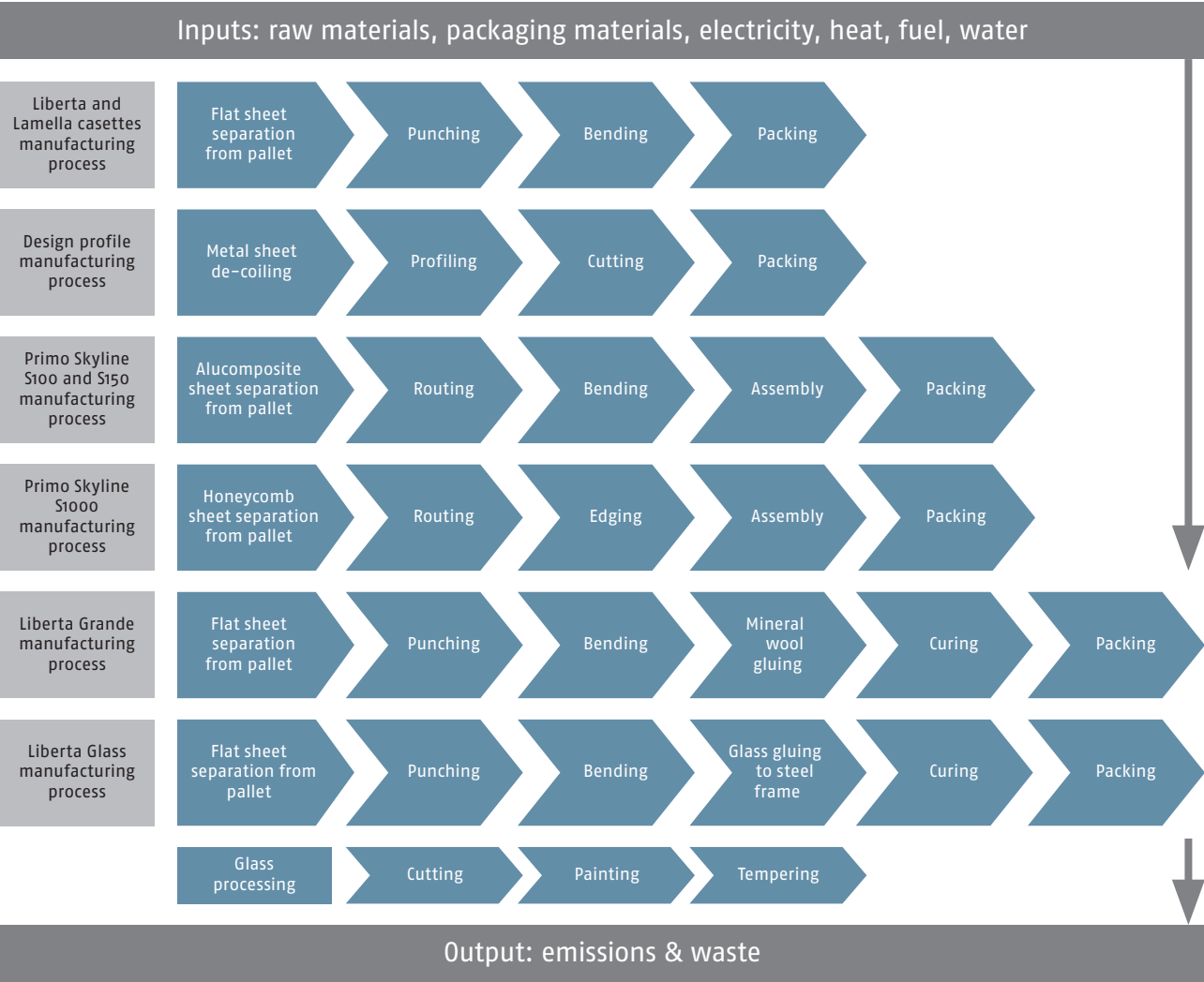
Figure 2. The production processes of façade cladding products
